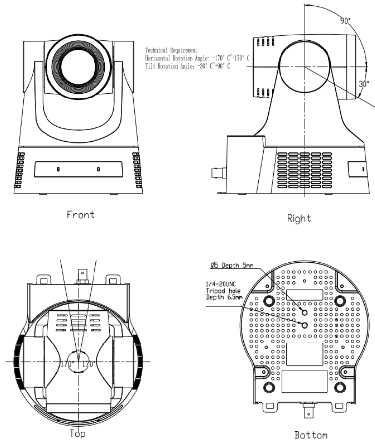
Figure 2.1 Product Dimension
