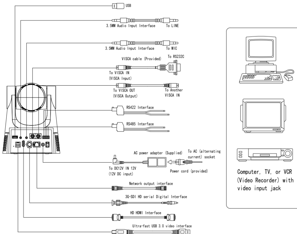
Figure 1.2 Wiring Diagram
