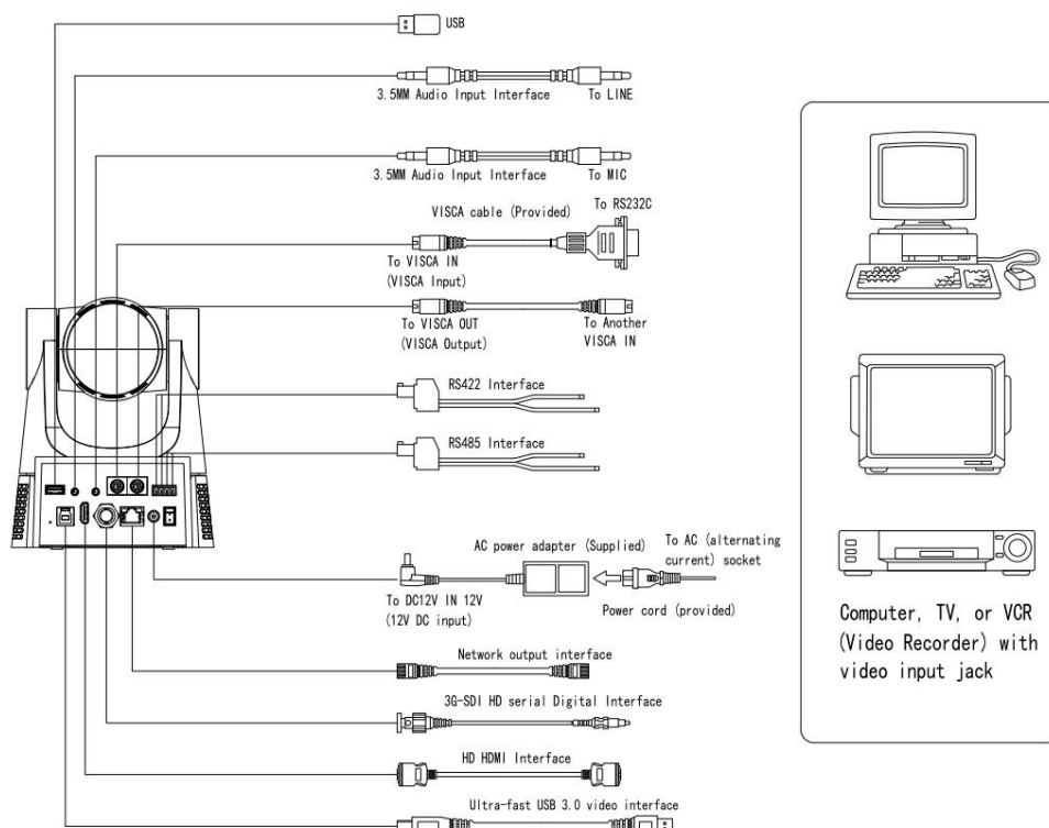
Figure 1.2 Wiring Diagram
