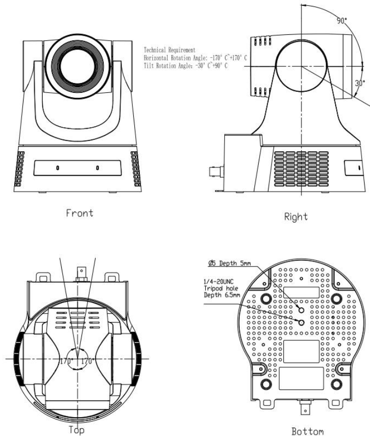
Figure 2.1 Product Dimension
